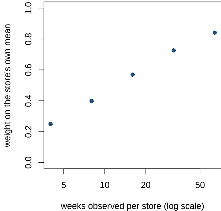
Weight \sigma_{\alpha}^2 / (\sigma_{\alpha}^2 + \sigma_{\varepsilon}^2 / n_s)
