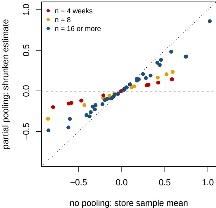
Shrinkage toward the grand mean
